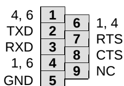
Figure 6: COM Connector
