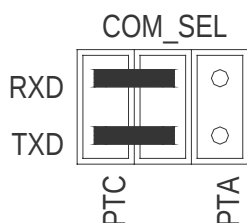
Figure 7: COM_SEL Option
